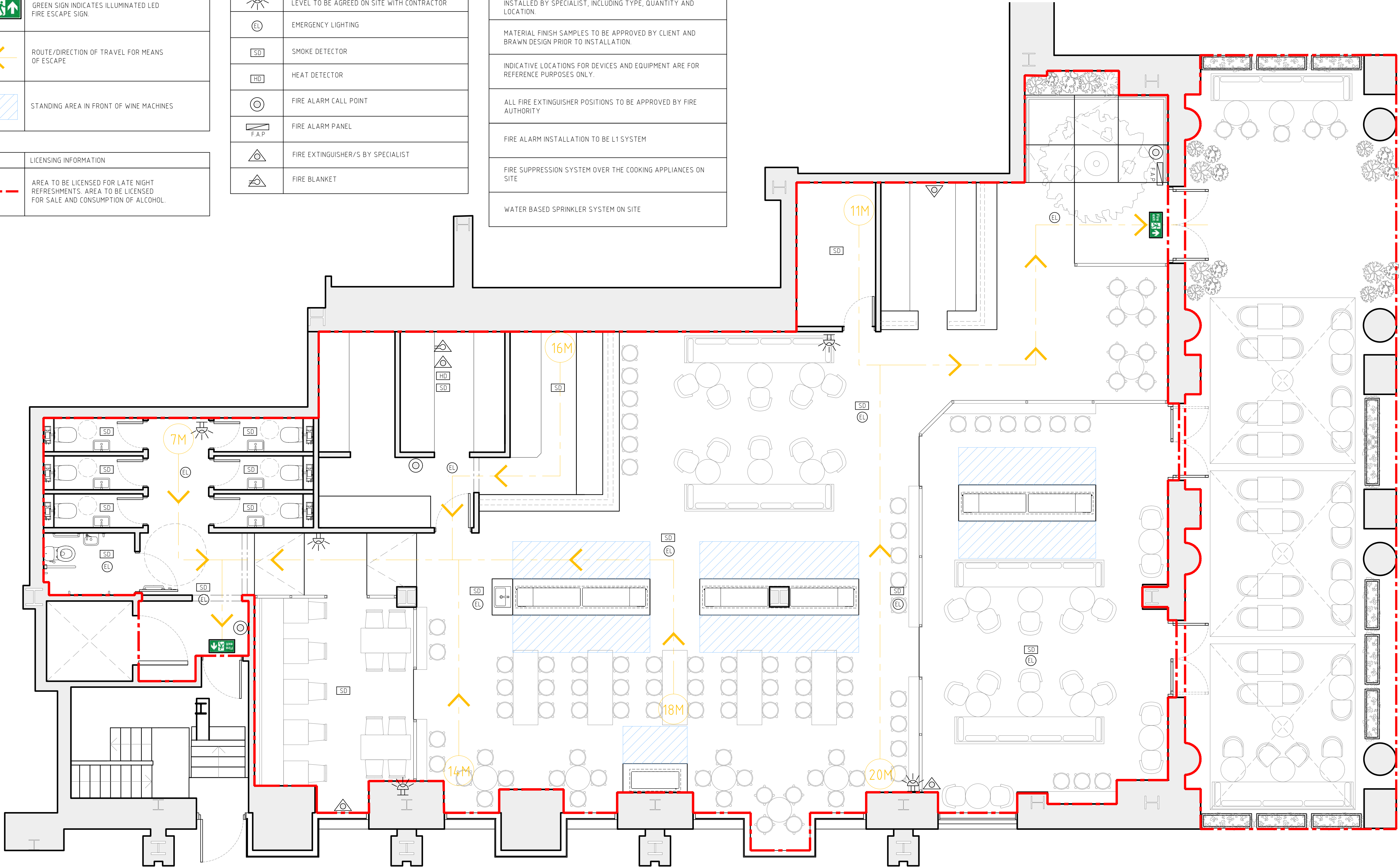
GROUND FLOOR GENERAL ARRANGEMENT SCALE 1:50
